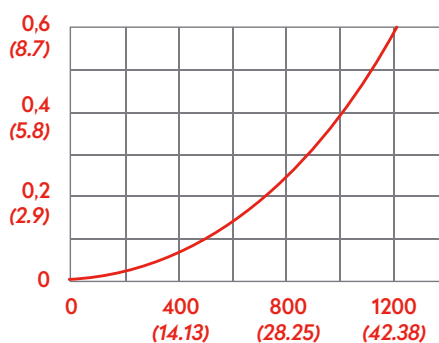
Air Flow Pressure drop bar (PSI)
