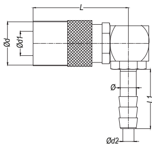
with standard hose tail 90°
