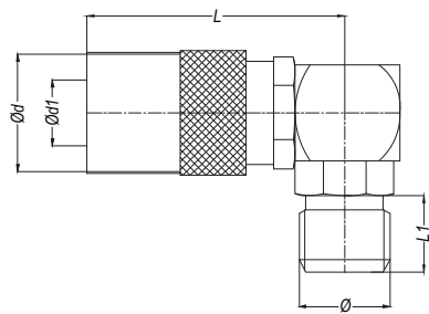
with male thread 90°
