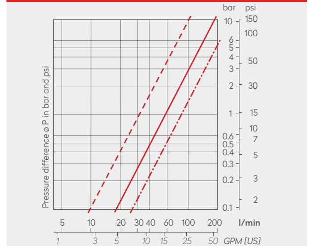
SV 2-Stage DN8 3/8" Performance Graph Water
